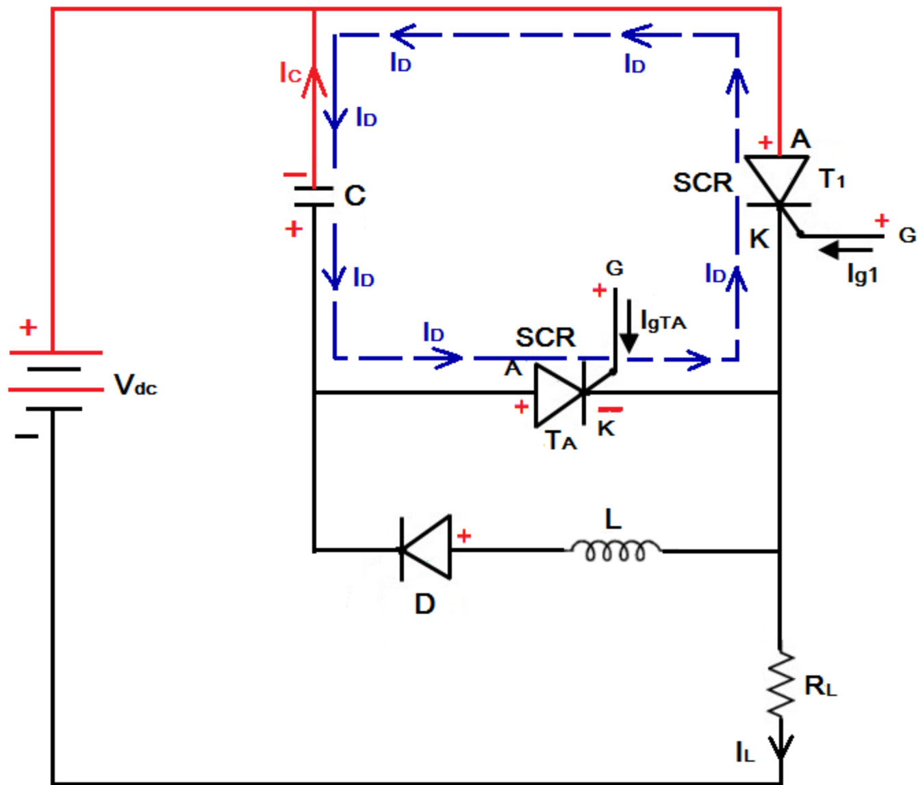
Class-D Commutation
