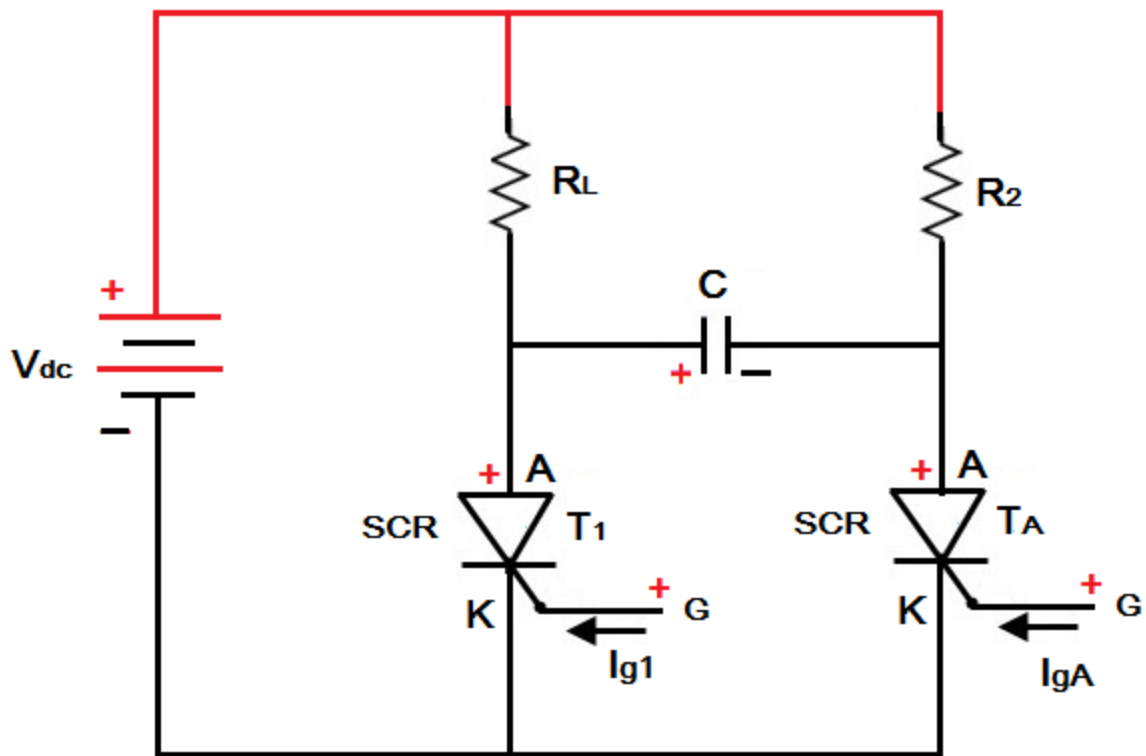
Class-C Commutation
