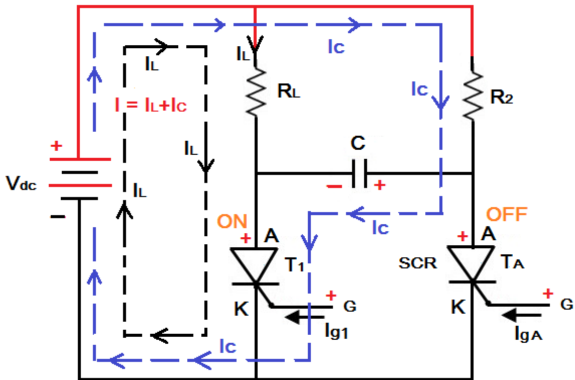
Simplified Diagram when SCR T1 ON
