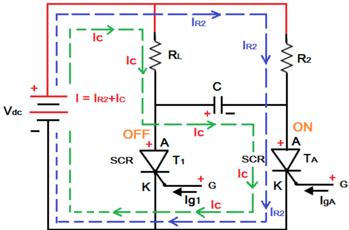
Simplified Diagram when SCR T_A ON
