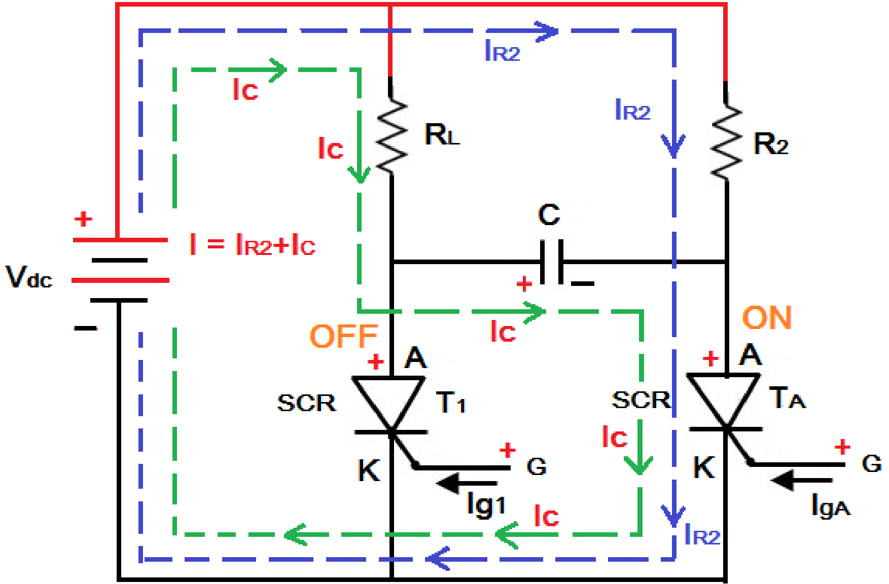
Simplified Diagram when SCR T A ON
