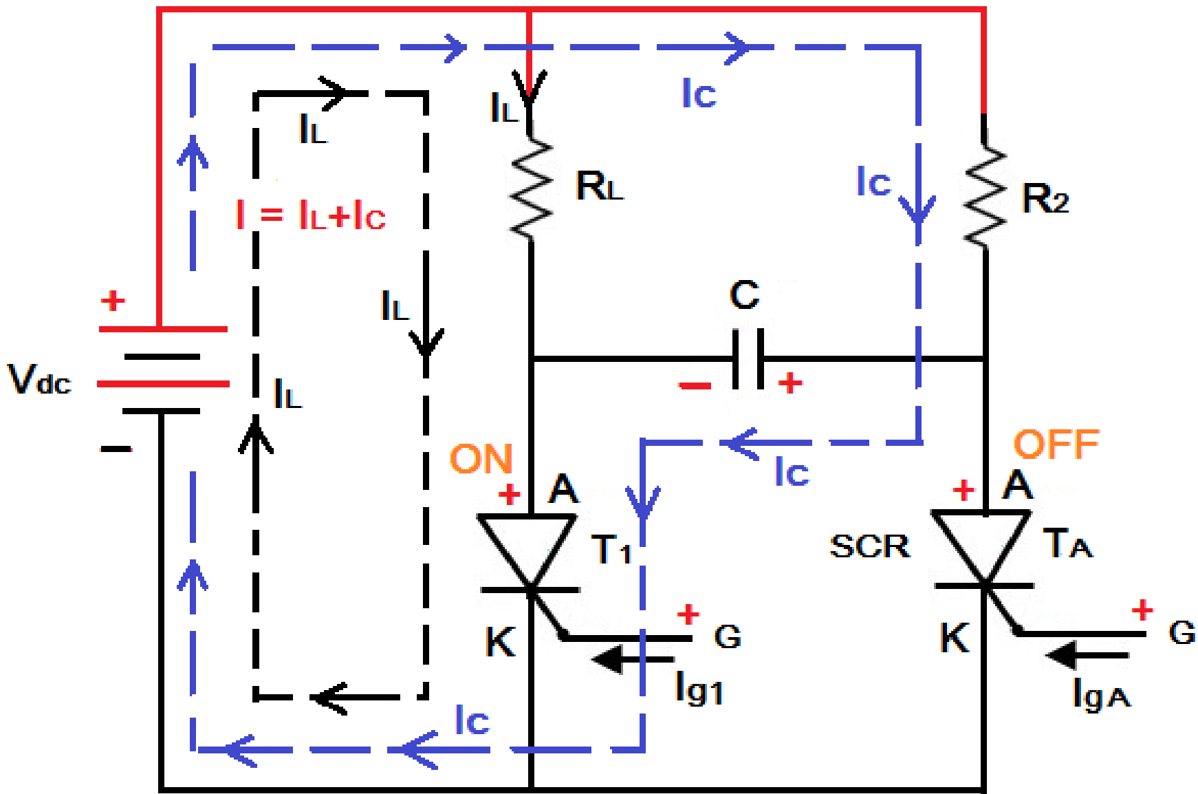
Simplified Diagram when SCR T1 ON
