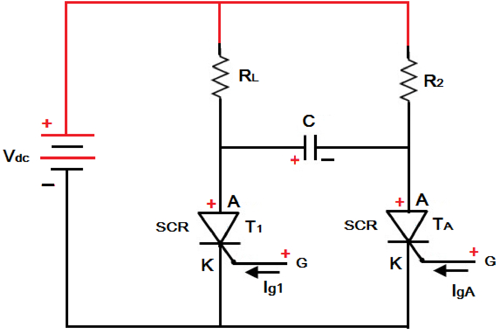
Class-C Commutation
