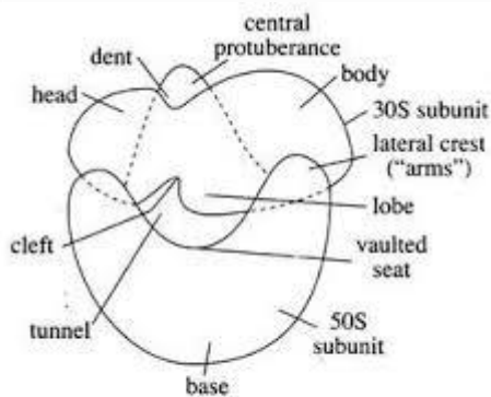
Fig. 3.17 : Stofler and Wittman's model of 70S ribosome.
