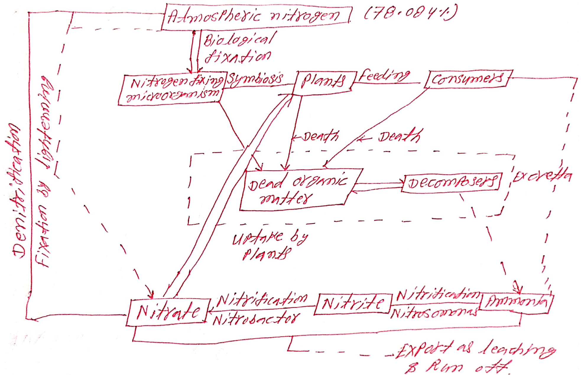
Fig:- Nitrogen cycle
