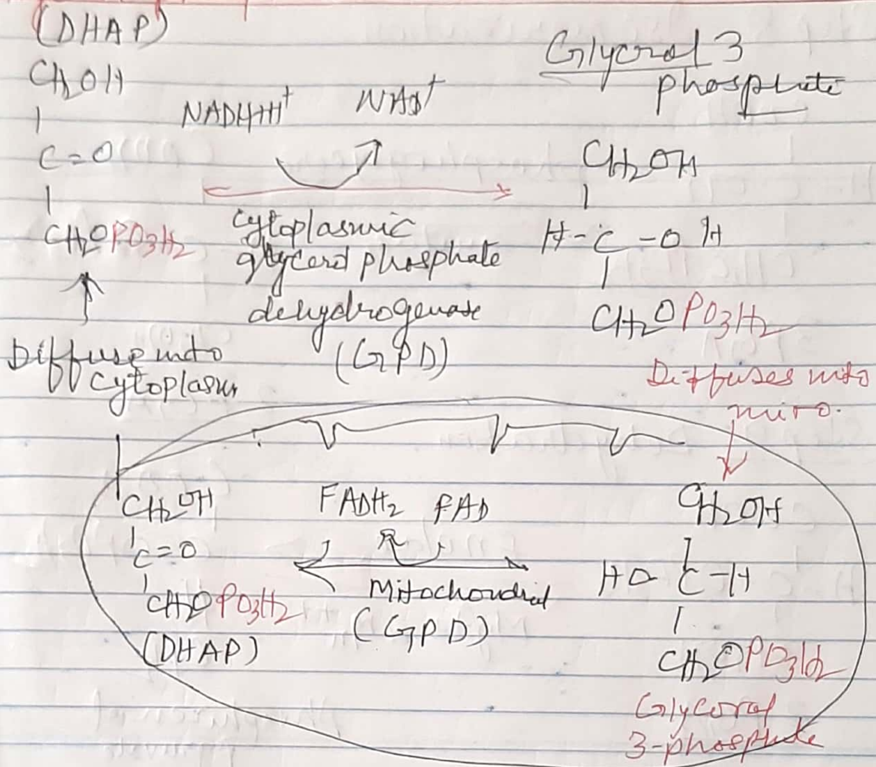
Fig - Glycerol phosphate shuttle
