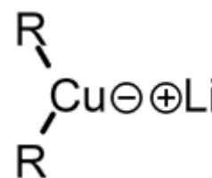
General structure of a Gilman reagent
