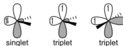
Singlet and triplet carbenes
